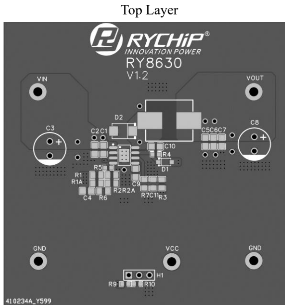
Sample Board Layout
