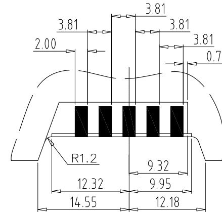
PCB LAYOUT PCB THICKNESS :1.4-1.7mm
