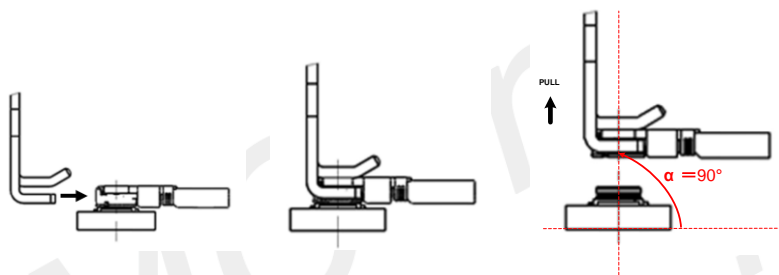
Figure 45: Use RF cable tool correct pull and push operation
