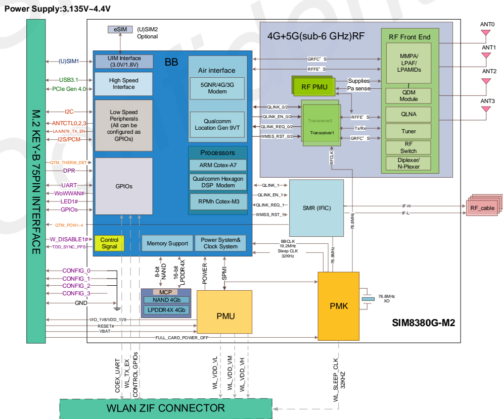
Figure 2: Block diagram
