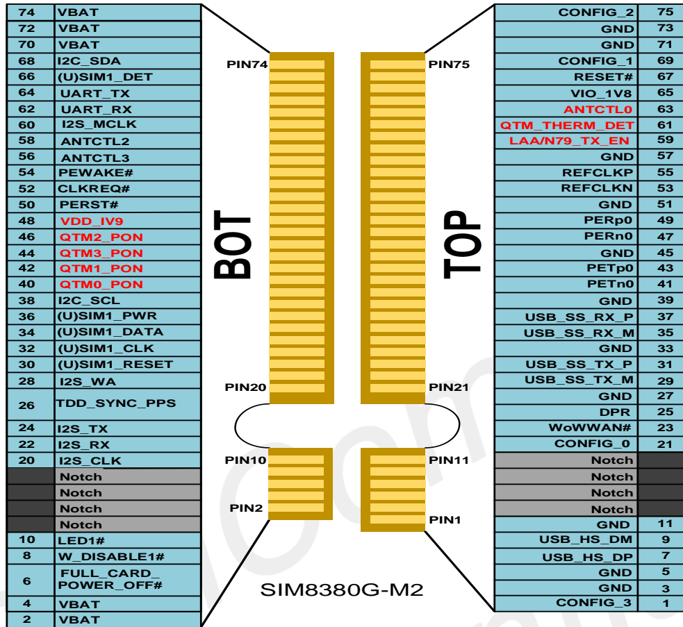
Figure 3: Pin assignment
