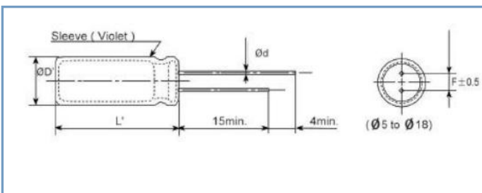
Radial Type
