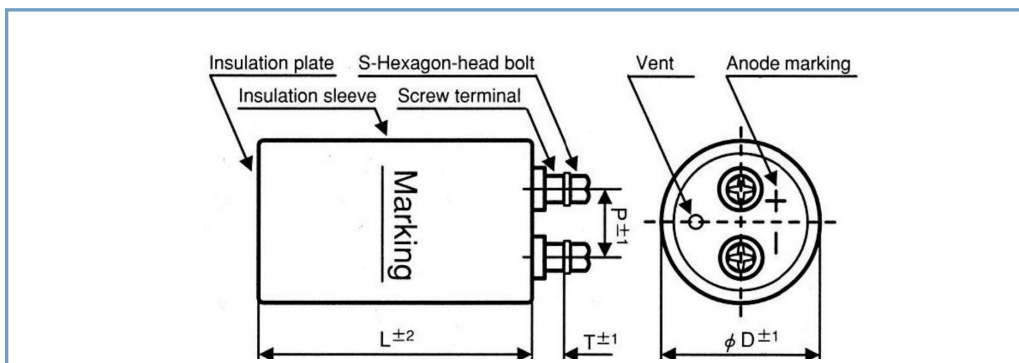
Screw Type
