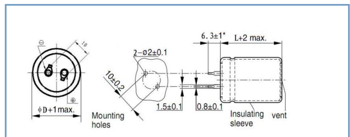
Snap-in Type
