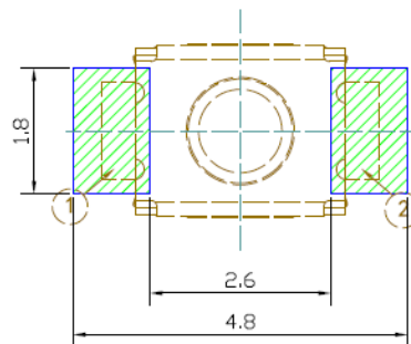
P. C. B MOUNTING PATTERN DIMENSION
