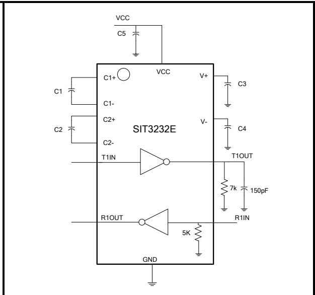
Fig 3 maximum swing rate test circuit
