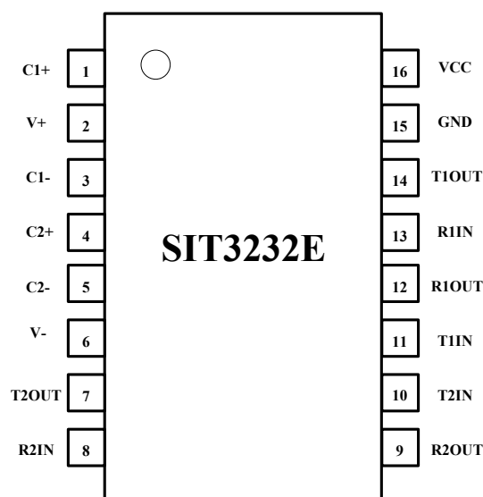
Fig 1 pin configuration
