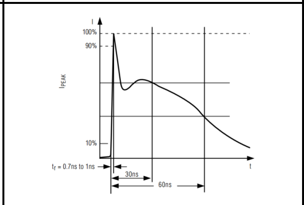
Fig 7 current waveform of IEC 1000-4-2 ESD
