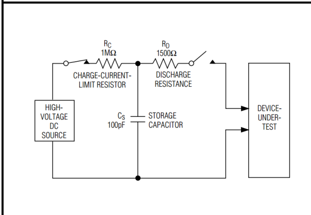
Fig 4 ESD test model of human body mode
