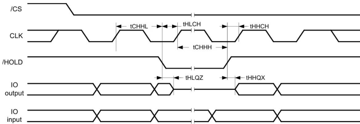
Figure 6-5 /HOLD Timing
