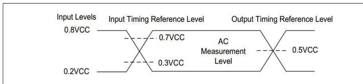
Figure 6-2 AC Measurement I/O Waveform
