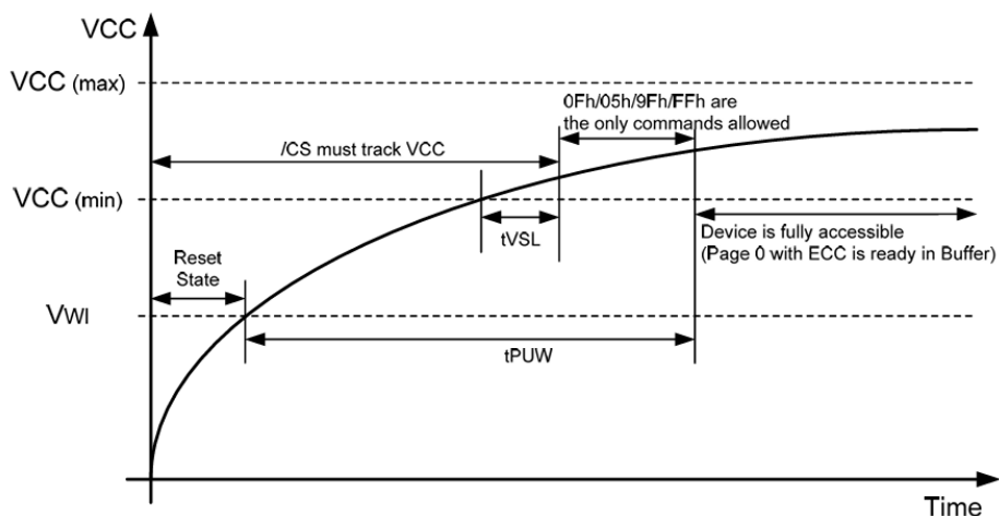
Figure 6-1 Power-on Timing
