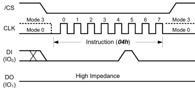
Figure 3-4 Write Disable (04h) Timing
