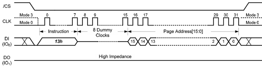
Figure 3-8 Page Data Read (13h) Timing
