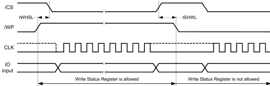
Figure 6-6 /WP Timing
