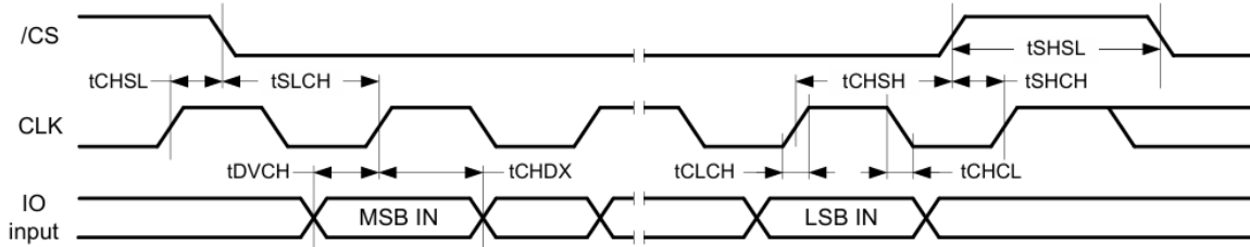
Figure 6-4 Serial Input Timing
