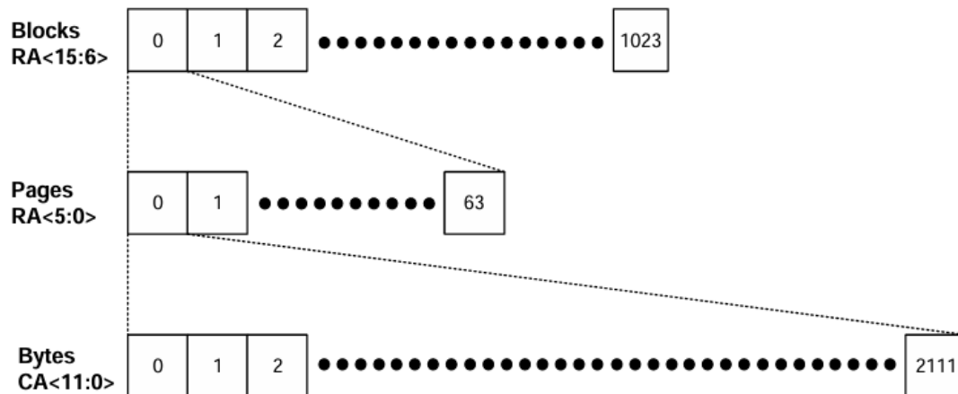
Figure 1-3 Memory Mapping
