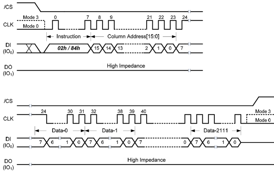
Figure 3-5 Load/Random Load Program Data (02h/84h) Timing
