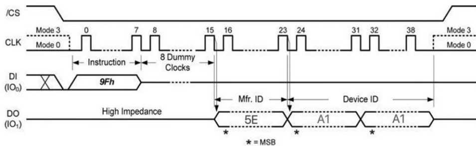
Figure 3-2 READ JEDEC ID (9Fh) Timing
