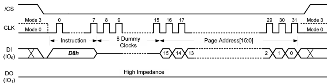
Figure 3-15 Block Erase (D8h) Timing
