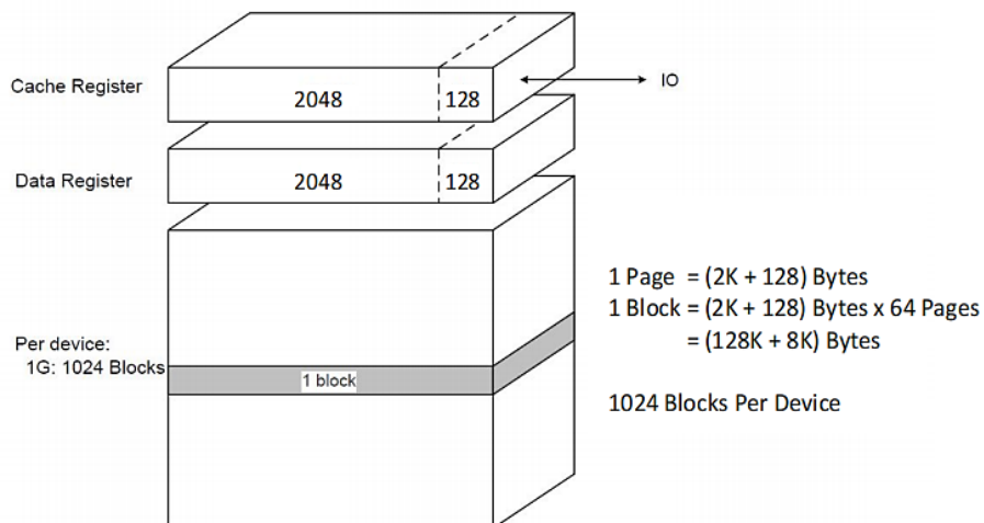
Figure 1-4 Array Organization 1 Gb
