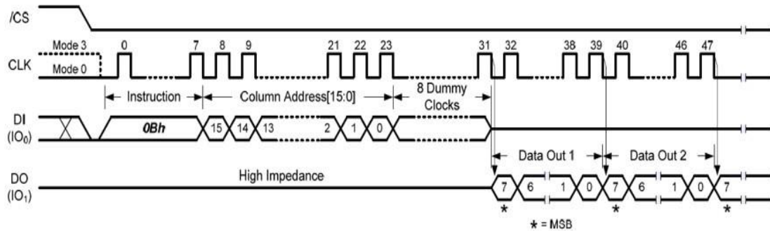
Figure 3-10 Fast Read (0Bh) Timing
