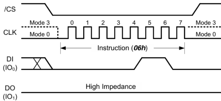
Figure 3-3 Write Enable (06h) Timing
