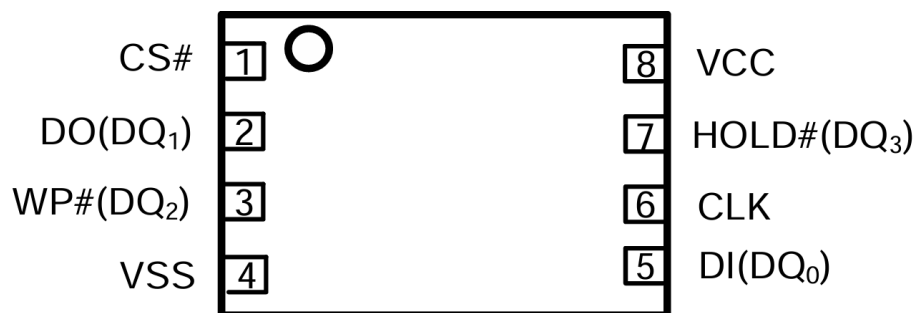
Figure 1-1 Pad Assignments
