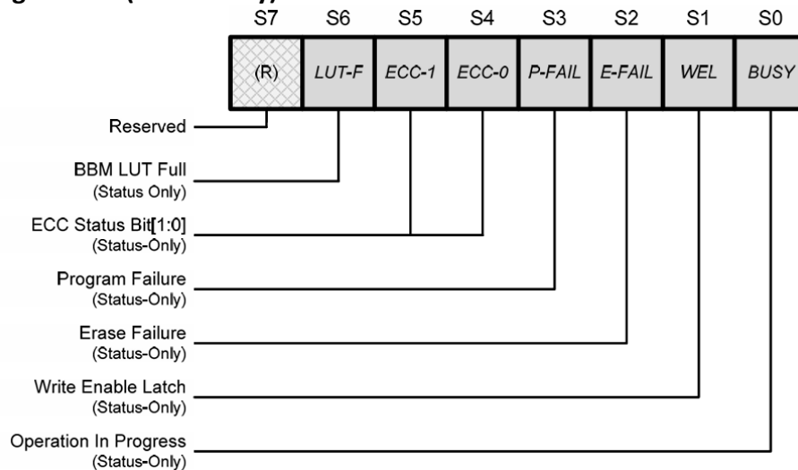
Figure 3-22 Status Register-3 (Address C0h)
