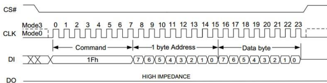
Figure 3-19 Set Features (1Fh) Timing
