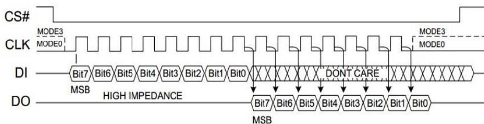
Figure 2-1 SPI Modes Supported
