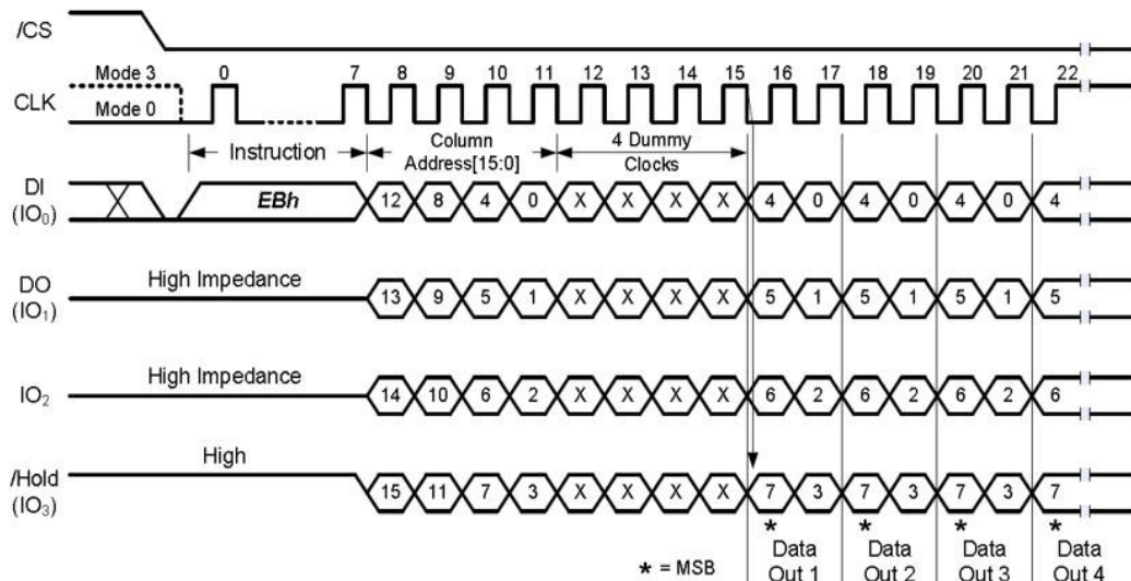
Figure 3-14 Fast Read Quad I/O (EBh) Timing
