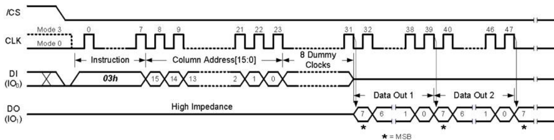
Figure 3-9 Read (03h) Timing
