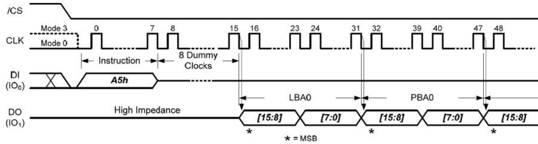
Figure 3-17 Bad Block Management (A5h) Timing
