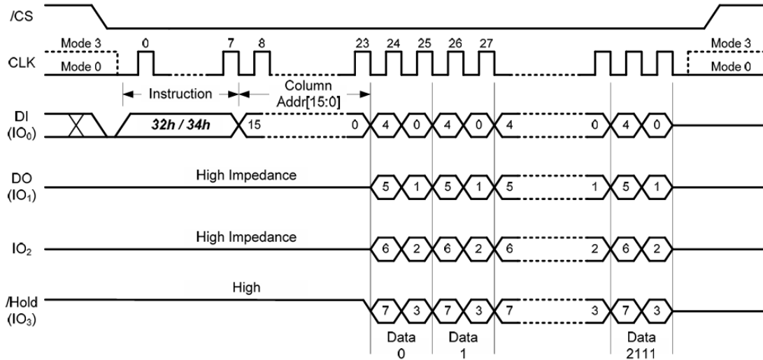
Figure 3-6 Quad Load / Quad Random Load Program Data Timing
