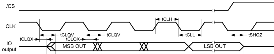
Figure 6-3 Serial Output timing
