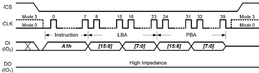
Figure 3-16 Bad Block Management (A1h) Timing
