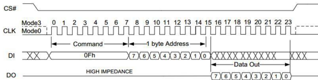
Figure 3-18 Read Feature (0Fh) Timing
