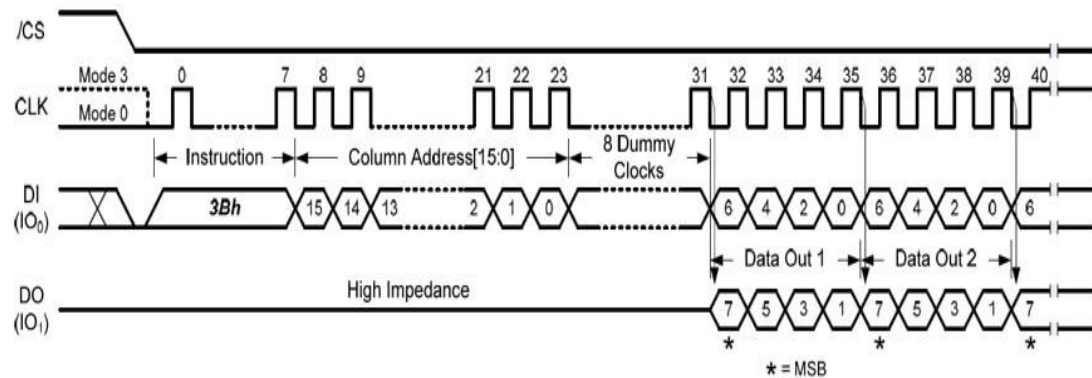
Figure 3-11 Fast Read Dual Output (3B) Timing
