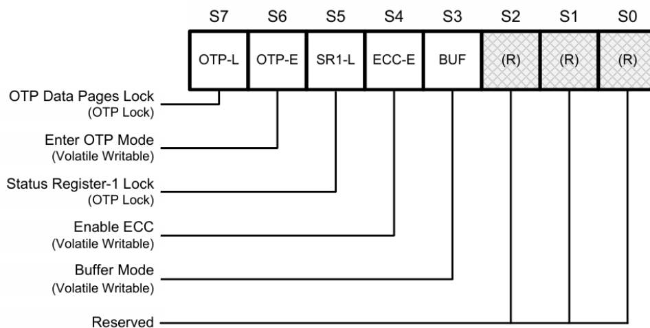
Figure 3-21 Configuration Register / Status Register-2 (Address B0h)
