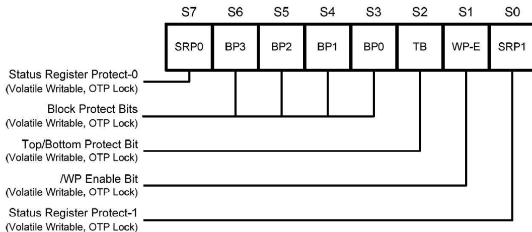
Figure 3-20 Protection Register / Status Register-1 (Address A0h)
