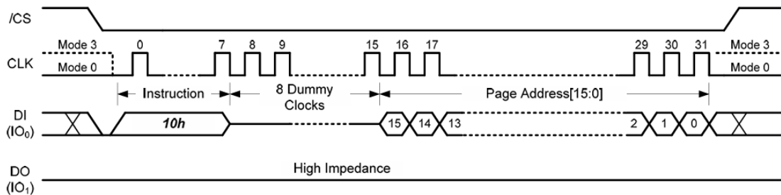
Figure 3-7 Program Execute (10h) Timing
