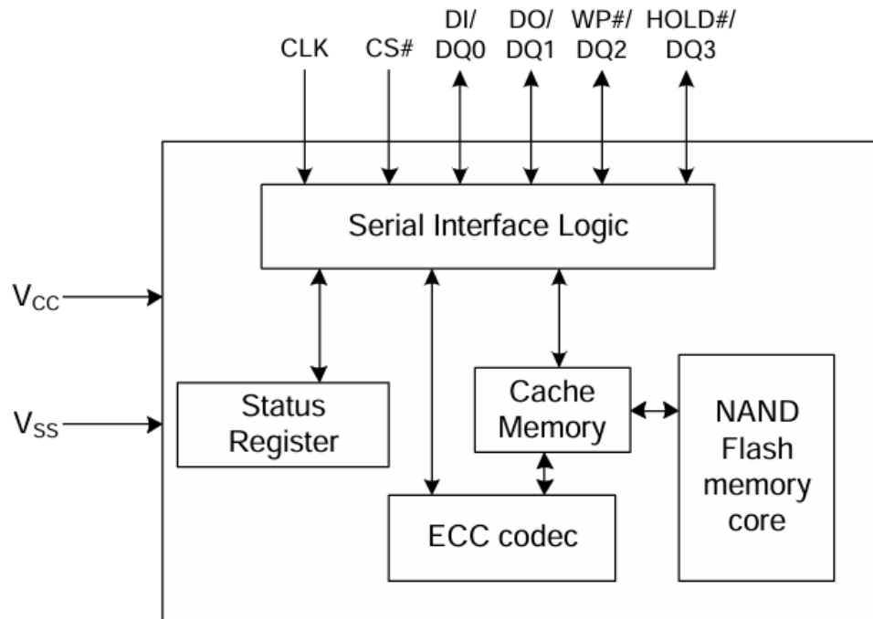
Figure 1-2 Memory Block Diagram
