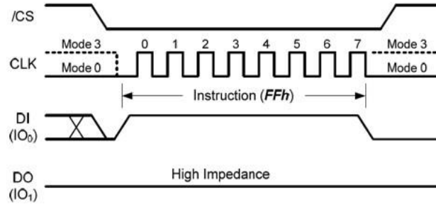
Figure 3-1 RESET (FFh) Timing
