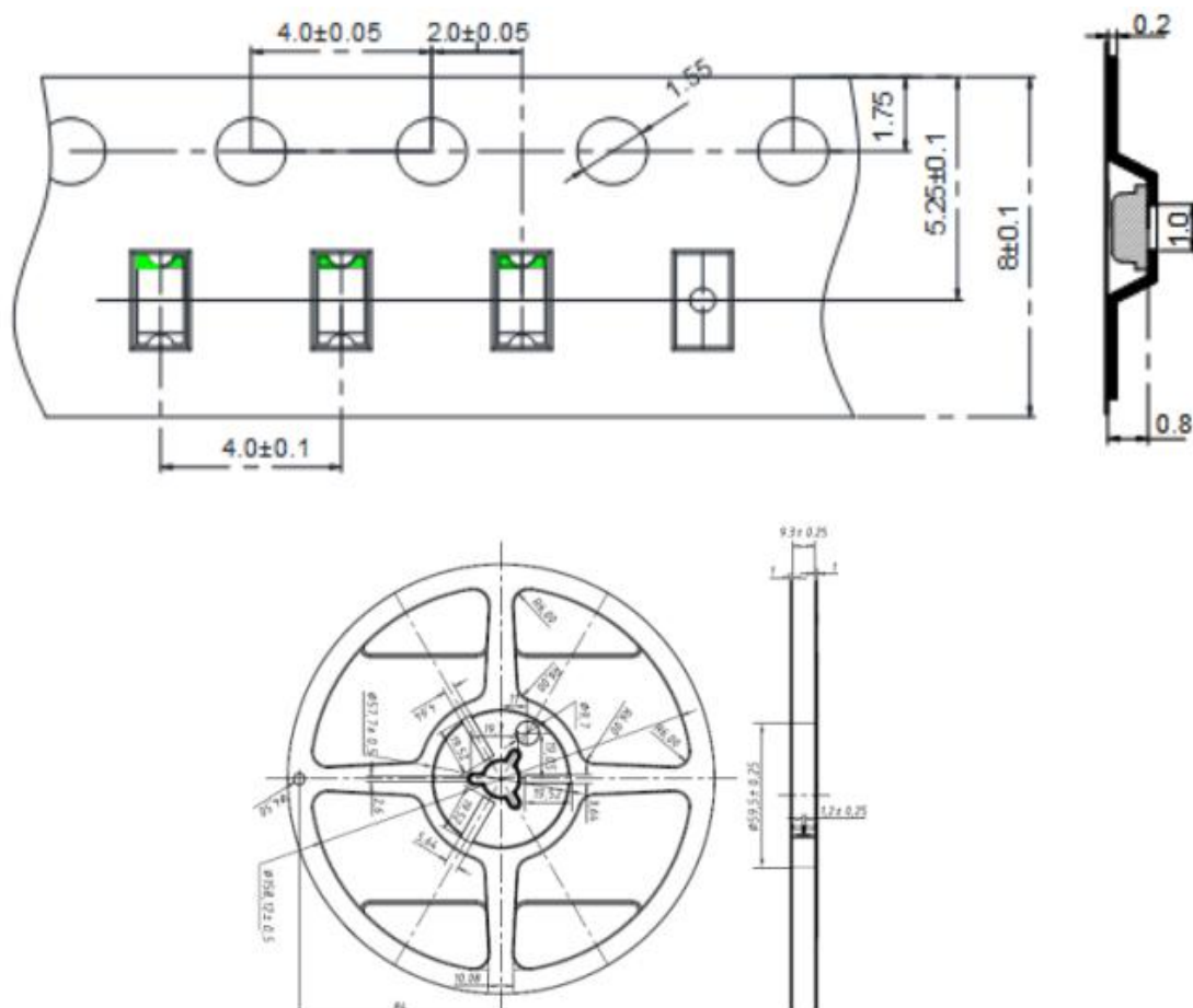
载带与圆盘尺寸 Belt and disk dimensions
