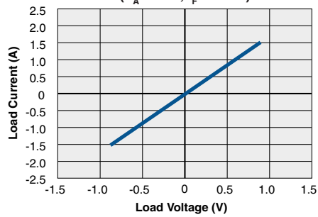
CPC1979 Typical Load Current vs. Load Voltage ( T_A = 25^\circ\text{C} , I_F = 10\text{mA} )
