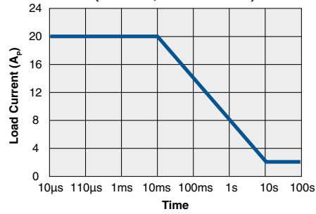
CPC1979 Energy Rating Curve (Free Air, No Heat Sink)
