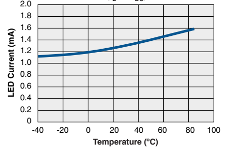
CPC1979 Typical I_F for Switch Operation vs. Temperature ( I_L = 1A_{DC} )
